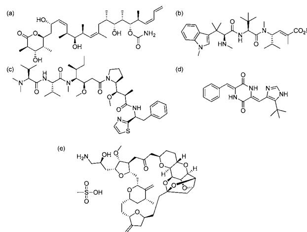
Figure 1. Chemical structures of tubulin binders. Marine natural products: (a) discordemolide, (b) hemiasterlin, (c) dolastatin 10. Synthetic compounds inspired by marine natural compounds: (d) plinabulin, (e) eribulin mesylate.
